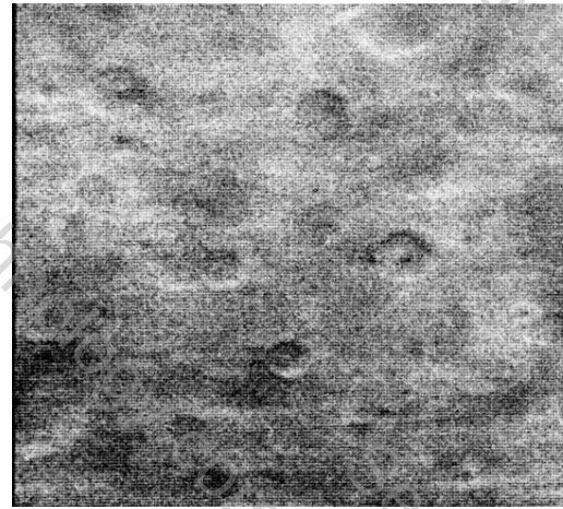
(6b) 1964, NASA Mariner 4
