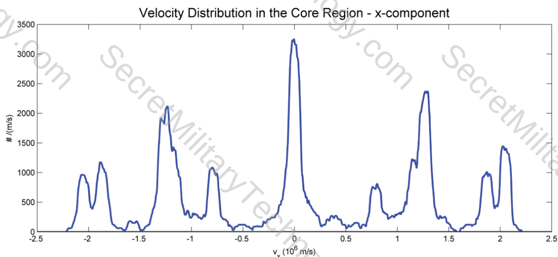
Figure 5.7: Velocity distribution in the x -dimension of ions in the core region, with one beamline aligned with x .
