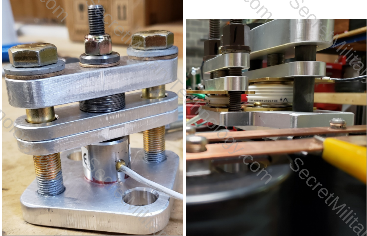
(a) Semiconductor clamp calibration using precision load cell.
