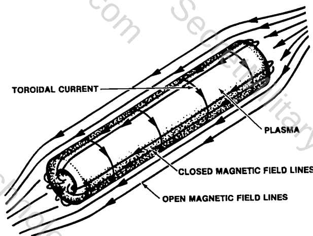
Fig. VI-1. Reversed-field configuration.
