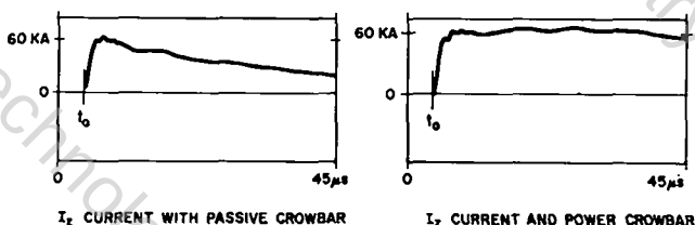
Fig. II-9. Comparison of ZT-S current waveforms with and without power crowbar.
