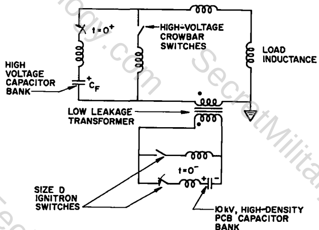
Fig. XVII-3. Basic ZT-40 power crowbar circuit.
