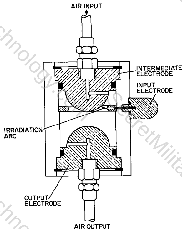
Fig. XVII-31. Inside-out trigatron peaking gap.
