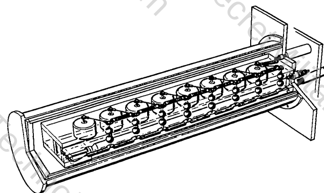
Fig. XVII-17. ZT-40 micromarx 200-kV pulse generator.
