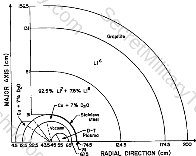
Fig. XVI-26. Two-dimensional RIGGATRON blanket model used for neutronics computations.
