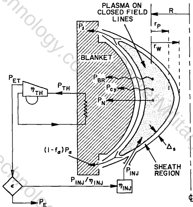
Fig. XVI-13. Schematic diagram of idealized, steady-state Tormac reactor energy balance.
