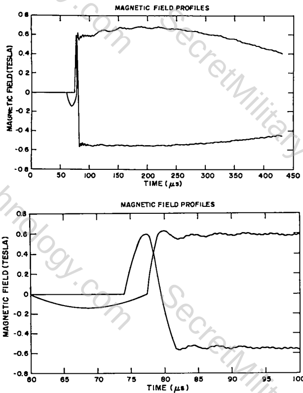
Fig. XVII-6. Representative Padua Mode waveforms.
