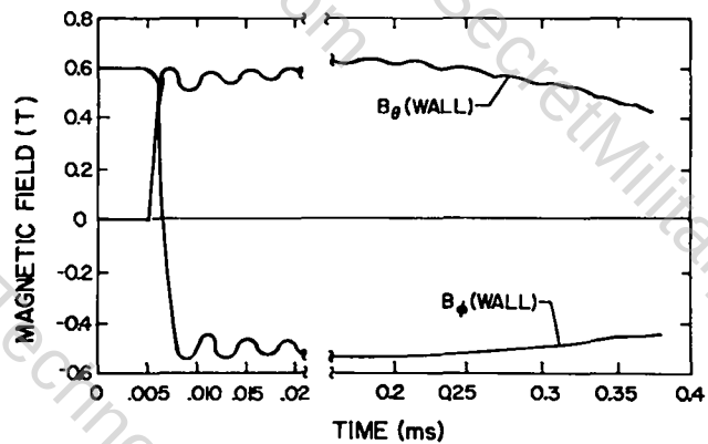
Fig. II-14. Numerical calculation of toroidal and poloidal currents vs time for a 12-feedplate design.
