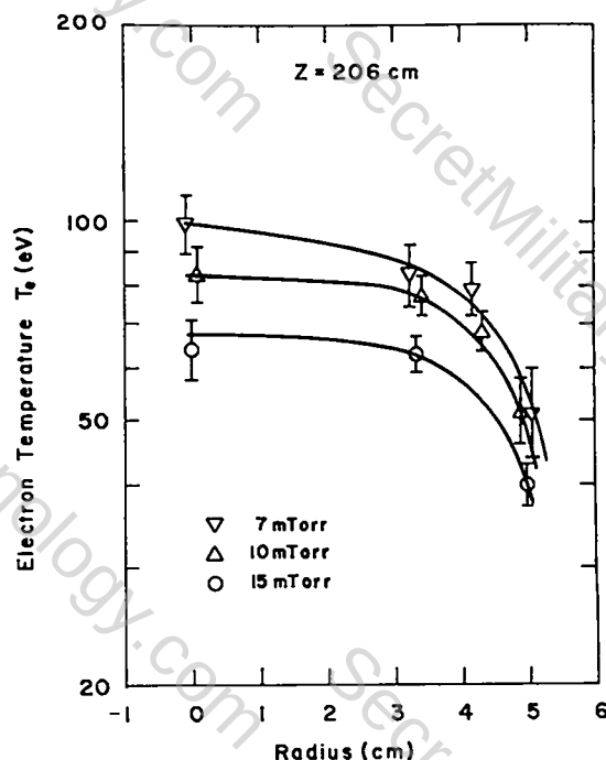
Fig. V-8. Electron temperature vs radius for three initial D_2 fills at a position near the end of the compression coil.
