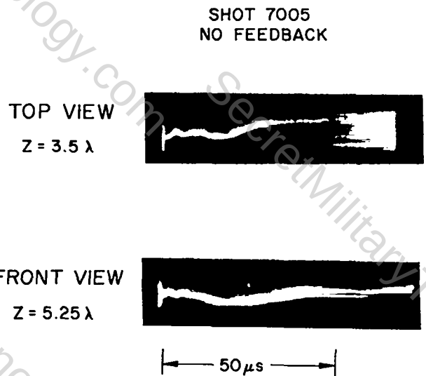
Fig. III-4. Streak photographs of plasma without feedback.
