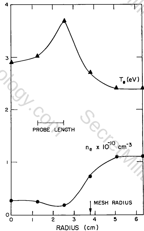
Fig. X-12. Electron density and temperature at 30.5 cm. from midplane vs radial position for 6.4-mm mesh spacing. Same discharge conditions as Fig. X-11.
