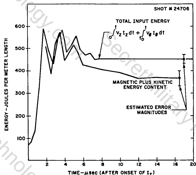
Fig. II-2. Curves of energy input and content vs time in ZT-S.
