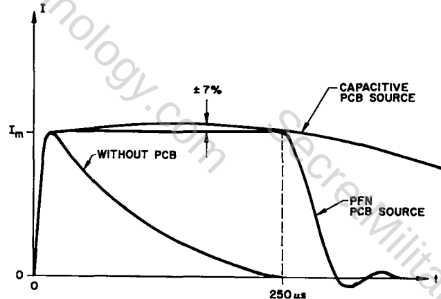
Fig. XVII-2. General ZT-40 current waveforms.
