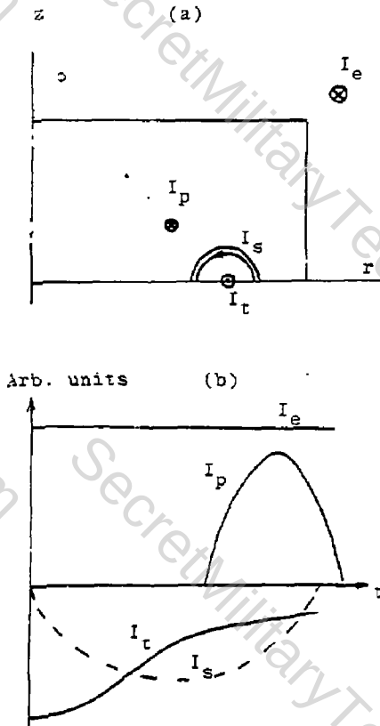
Fig. 1. (a) Schematic diagram of spheromak.
