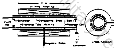
Fig. 2 Experimental Apparatus
