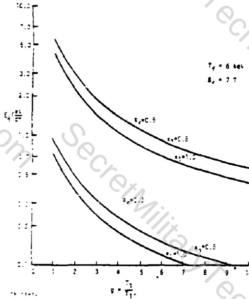
Figure 2. Electric Field Reduction With Axial Compression. Field Required to Achieve T_f = 6 keV at fill factor X_f with 7 Tesla Magnetic Field. Length Compression Factor = 3. X_1 = radial fill factor immediately after reconnection.
