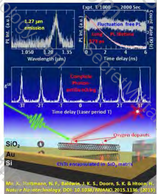
Figure 3. Illustration of single photon emission behavior arising from carbon nanotubes doped in a solid-state process developed in the project. Exciton localization at dopant trap sites yields extended emission lifetimes and complete antibunching at room-temperature as signature of single photon emitter.
