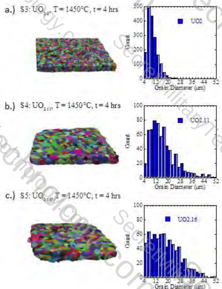
Figure 1. Grain map and grain size distribution for a.) UO 2 , b.) UO 2.11 , and c.) UO 2.16 .
