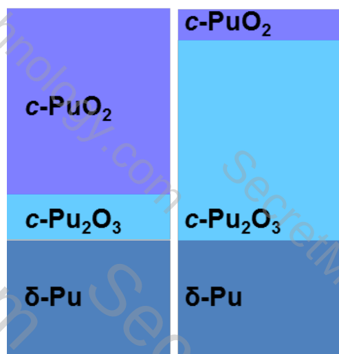
Figure 1. Historical depiction of oxide products formed on delta-plutonium under ambient (left) and UHV (right) conditions ("" refers to the crystalline form).
