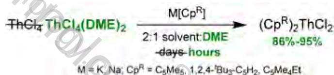
Figure 1. General scheme depicting the synthesis of metallocene thorium dichlorides from \text{ThCl}(\text{DME}) ; shows that the addition of DME to a reaction mixture improves synthetic efficacy of \text{ThCl}(\text{DME}) .
