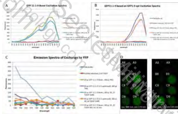
Figure 5. Light exchange experiment with caged GFP 11-1-9-tev-10 constructs. A. Excitation spectra of GFP11-1-9-tev-10 Boxer version with controls and sample with excess sulfate reductase_10 T203Y (SR_10) added to solution. There is a marked shift toward 510 nm as excitation max in 405 nm exposed sample (purple trace). B. Excitation spectra of GFP11-1-9-tev-10 based on GFP1-9 optimized with controls and samples with excess SR_10 T203Y. No shift in excitation sample was noted as compared to sample in dark or control GFP11-1-9-tev-10. C. Emission spectra in light exchange experiment. Only the GFP11-1-9-tev-10 boxer construct exposed to 405nm light after excess SR_10 T203Y was added had an increase in emission over the other samples. D. Plate photographed after excitation at 488 nm, emission at 510 nm (exposure time 1/15 sec). Second image is the same plate photographed after excitation at 520 nm, emission at 550 nm (exposure time 4 sec). Wells correspond to: A8 200 \mu L TNG buffer; A9 20 \mu L TNG, 180 \mu L SR_10 T203Y; B8 20 \mu L Boxer, 180 \mu L TNG; B9 20 \mu L 11-1-9-rev-10 1-9 opt, 180 \mu L TNG; C8 20 \mu L Boxer, 180 \mu L SR_10 T203Y kept in dark; C9 20 \mu L 11-1-9-rev-10 1-9 opt, 180 \mu L SR_10 T203Y kept in dark; D8 20 \mu L Boxer, 180 \mu L SR_10 T203Y after 15 minutes 405 nm exposure; D9 20 \mu L 11-1-9-rev-10 1-9 opt, 180 \mu L SR_10 T203Y after 15 minutes 405 nm exposure. D8 has a marked increase in yellow fluorescence.
