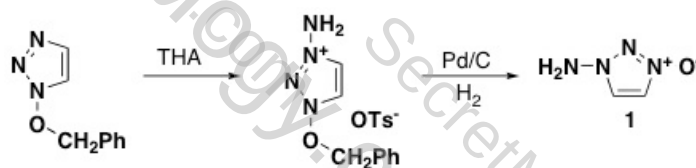
Figure 3. An alternate synthesis route to DPX-2 ( 1 ) was pursued as the original process was low yielding. In this alternate route, 1-(benzyloxy)-1,2,3-triazole was aminated with tosylhydroxylamine (THA), to provide the N-amino intermediate. This intermediate compound was converted to DPX-2 ( 1 ) using hydrogen gas in the presence of a palladium catalyst. Although this route requires two steps, it is more efficient than the original process to prepare DPX-2 ( 1 ).
