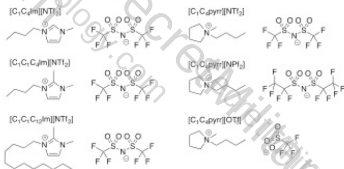
Figure 1. Ionic liquids synthesized and purified for gas absorption and N reduction studies.
