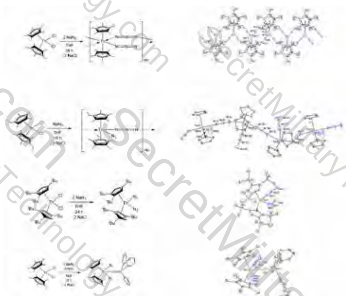
Figure 5. Syntheses of metallocene thorium diazides with corresponding X-ray crystal structures on the right. Trend: smaller ancillary ligands multinuclear complexes ( 1 ), while larger ancillary ligands mononuclear complexes ( 4 ).
