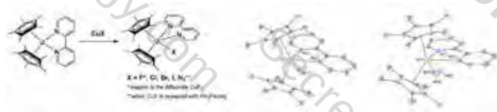
Figure 3. General scheme for the synthesis of (CMe)UX(bipy). X-ray crystal structures of (CMe)UBr(bipy) (structures for X = F and Cl are analogous) and (CMe)U(N 3 )(bipy).
