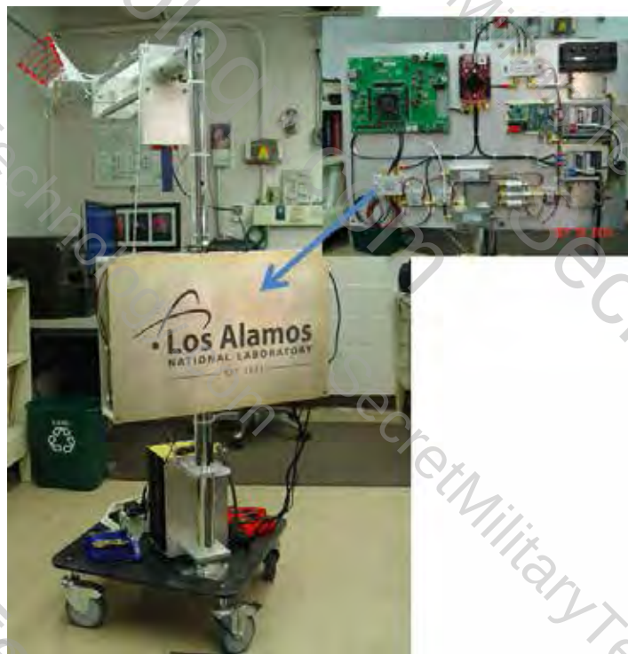
Figure 4. Our 1-GHz, 100-MHz bandwidth CDMA SAR hardware.
