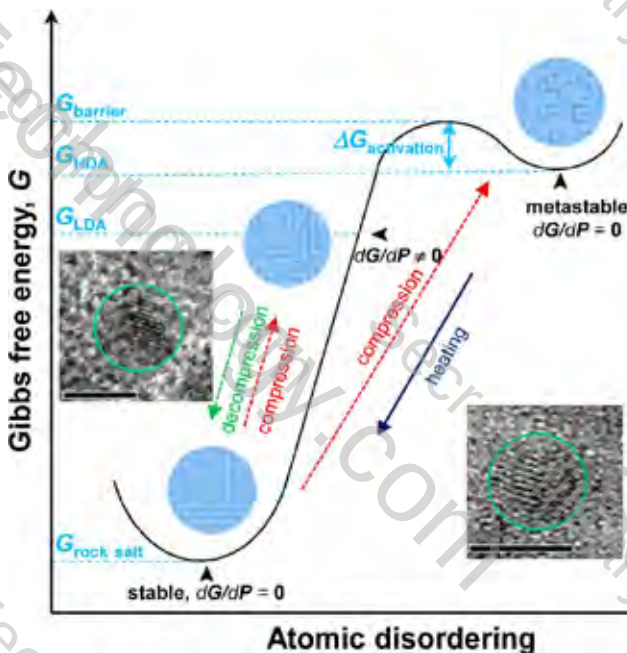
Figure 2. Schematic diagram showing the Gibbs free energy relation of the phase transitions observed in PbTe NPs and HRTEM images of the samples recovered from 15.6 GPa (left inset) and from 19.7 GPa at the initial stage of electron beam irradiation (right inset). The scale bars in both images represent 5 nm.
