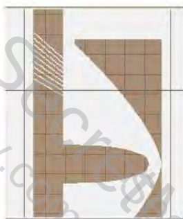
Figure 4. SIMION model showing a shaped pinhole plate and cone-like structure at the filter plate center. The pinhole is located above the center of the cone, and only a limited number of filter plate channels are shown.
