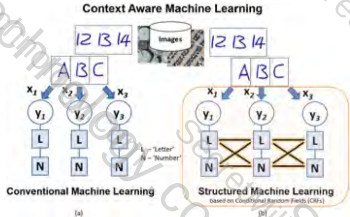
Figure 1. Illustration of context aware machine learning. (a) Conventional machine learning approaches classify input observed entities described with feature vectors x(i) independently of each other. (b) Our project focused on context aware structured machine learning approach based on conditional random fields (CRFs). CRF-based approach classifies input observed entities jointly (collectively) by exploiting dependencies y(i)-y(j) in the output domain, i.e. labeling of objects impacts each other interpretation. Context aware recognition of the central object y(2) is primed by how the adjacent objects y(1) and y(3) are recognized. y(2) is most likely to be "B" when its neighbors are recognized as "letters". y(2) is most likely to be "13" when its neighbors are "numbers."
