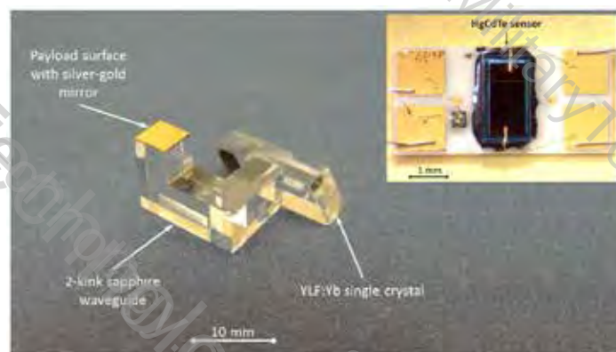
Figure 4. Picture of assembly consisting of a high-purity ytterbium-doped yttrium-lithium-fluoride (YLF:Yb) crystal and a two-kink sapphire waveguide. The YLF:Yb crystal input and output faces were cut at Brewster's angle in order to minimize reflection losses for the pump laser. The sapphire crystal was attached to the YLF:Yb crystal by a diffusion-bonding process that eliminated the use of adhesives, which could introduce parasitic heating. The two-kink sapphire waveguide provided a good thermal link between the crystal and the payload while preventing light from the crystal to reach the payload. A silver-gold mirror was deposited at the end of the sapphire waveguide for additional light rejection. The mercury-cadmium-telluride (MCT) infrared sensor (pictured in the inset) was mounted on top of the gold mirror.
