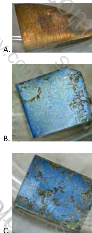
Figure 2. Pu with 1.9 at. % Ga after one month of exposure to dry air (A); wet air (B), and wet argon (C).
