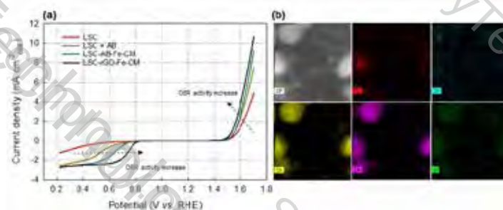
Figure 5. (a) ORR/OER activities of LSC and modified-LSC catalysts: LSC+AB, LSC-AB-Fe-CM, and LSC-rGO-Fe-CM. (b) Elemental EDS mapping from LSC-rGO-Fe-CM bi-functional catalyst.
