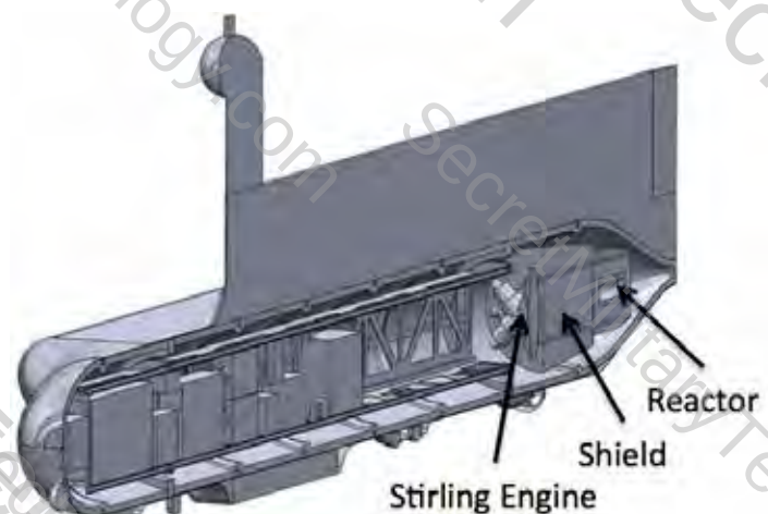
Figure 2. Shielding Study for Neutrons Dose for a Surfaced AUV.
