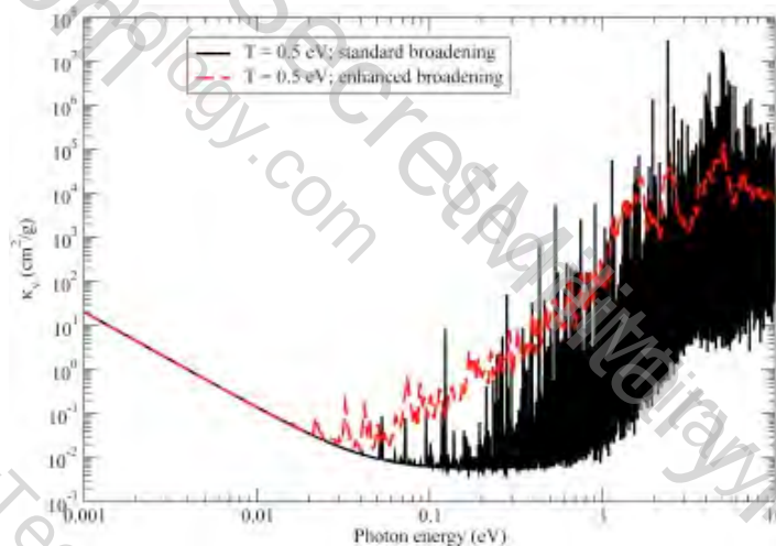
Figure 4. Monochromatic opacity of samarium (Sm, Z=62 ) over a broad range of photon energies. Our new local thermodynamic equilibrium (LTE) calculations show that line-rich spectra of heavier elements such as lanthanides increase the opacity in the visual and infra-red range by several orders of magnitude. The effect strongly impacts theoretical predictions of the electromagnetic emission from neutron star mergers widely anticipated to become the first directly detected gravitational wave (GW) sources. Early detection of optical counterparts to GW sources is currently a topic of intense interest both at LANL and across the astrophysics community.
