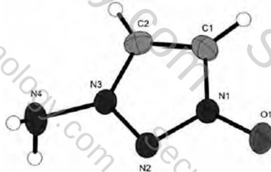
Figure 2. In order to confirm the molecular structure of 1 , crystals suitable for x-ray crystallographic analysis were grown from nitromethane solvent. This figure confirms our proposed structure and displays the molecule as it appears in the crystal structure. Non-H atomic displacement ellipsoids are 50% probability.
