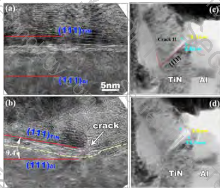
Figure 2. (a) and (b) HRTEM images of the Al-TiN interface before and after indentation. The red lines indicate the {111} plane. (c) and (d) Initiation and propagation of the crack II. The Al layer near the crack II does not fracture and the layer thickness reduces from 6.1 nm to 3.8 nm.
