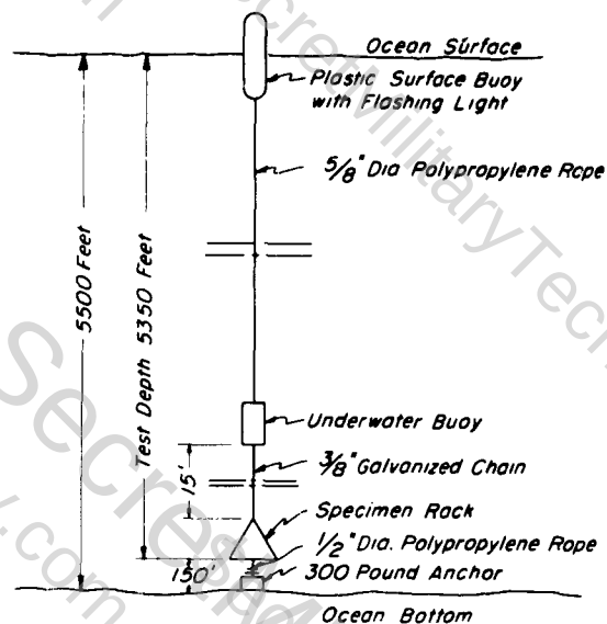
Schematic of deep-sea corrosion exposure system.
