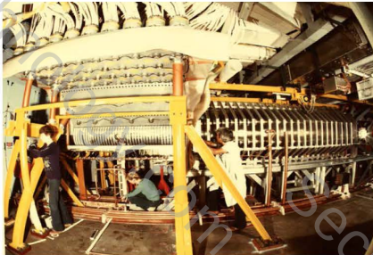
LANL FRX-C/T theta pinch (left) and dc magnet coils surrounding the translation chamber (right)
