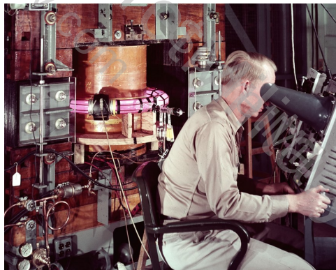
James Tuck, Perhapsatron, 1953
