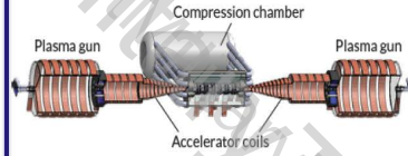
Helion Energy Redman, WA
